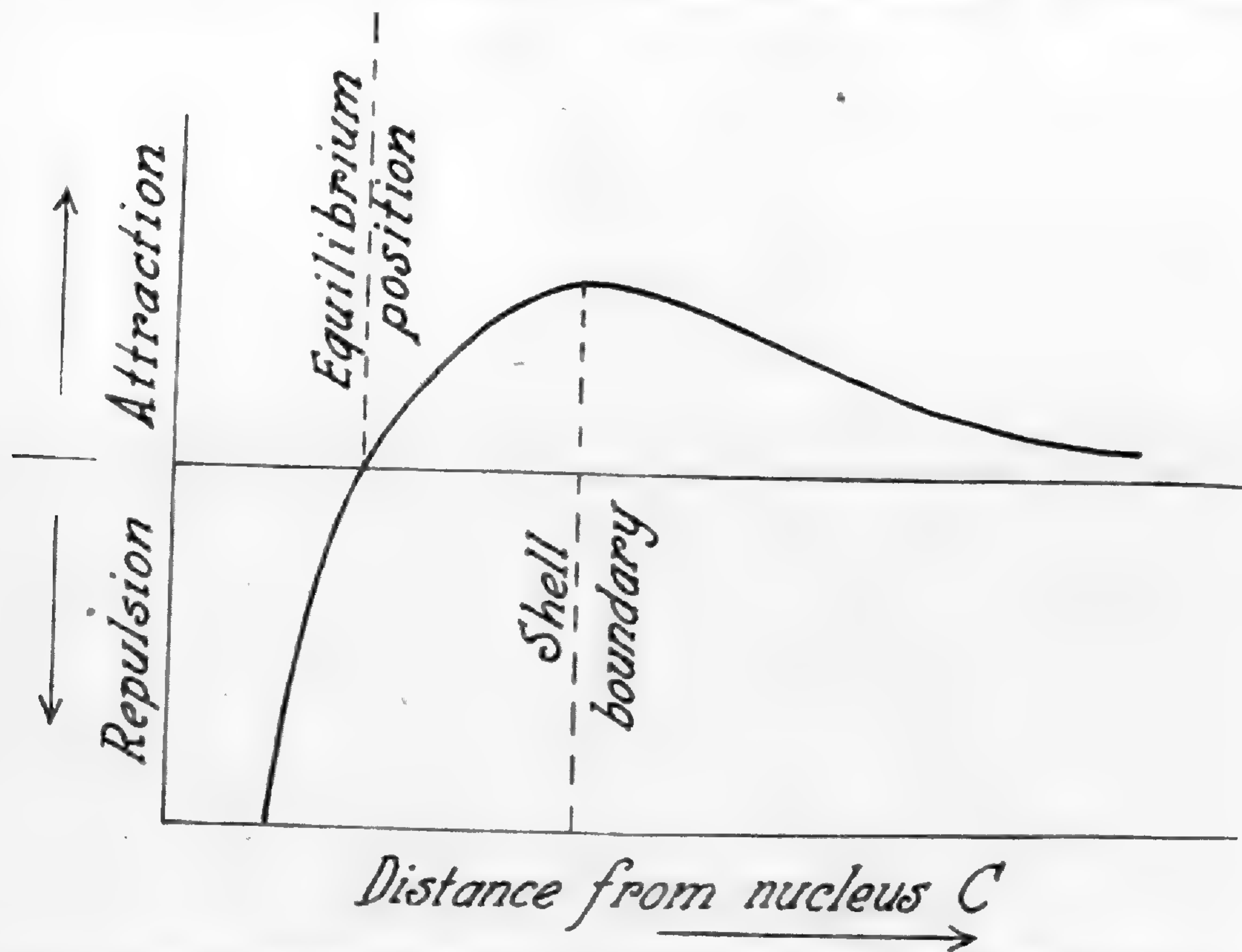
FIG. 1. Forces of restitution acting on an unshared shell electron, upon radial displacement.
